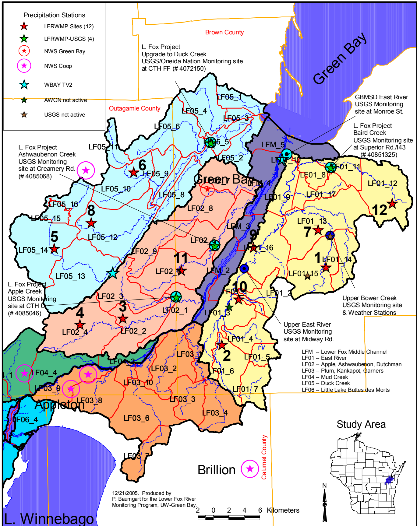
Rain Gauges in the Lower Fox River Basin, including those installed through the Lower Fox River Watershed Monitoring Program (LFRWMP, 16 total gauges).
